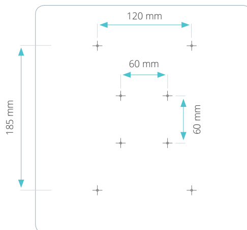
Mounting hole dimensions
